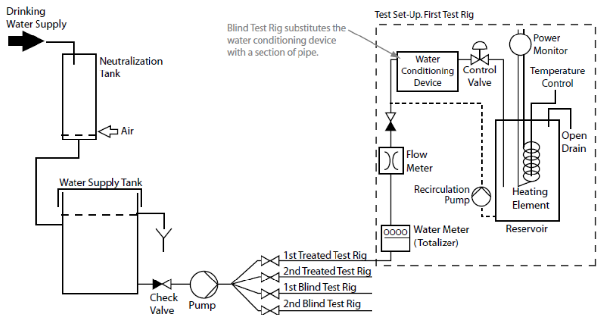
FIGURE 14: DVGW-W512 SCHEMATIC
