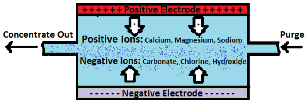
FIGURE 10: CDI BACKWASH
