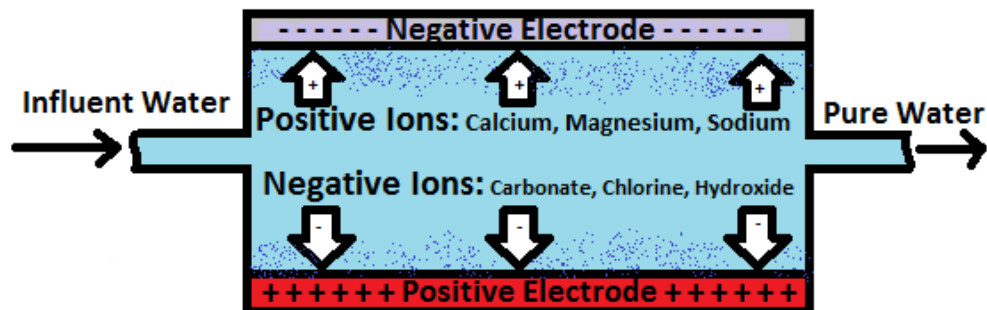
FIGURE 9: CDI REGENERATION
